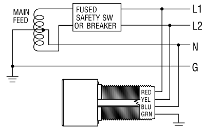
SINGLE PHASE, 3W + GND
