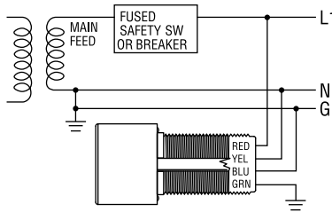
SINGLE PHASE, 2W + GND
