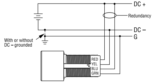
DC SINGLE SOURCE, 2W + GND
