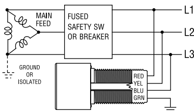
THREE PHASE DELTA, 3W + GND
