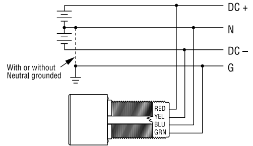
DC SPLIT SUPPLY, 3W + GND
